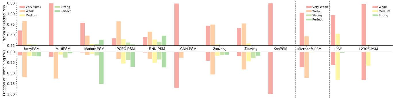
(a) Password score distributions (on Weibo) of leading PSMs under the brute-force guessing strategy.
