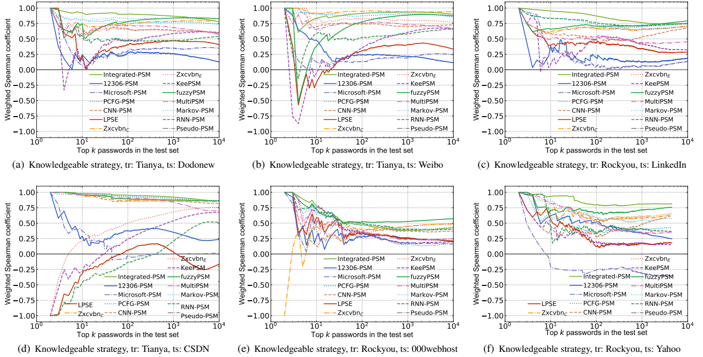
Figure 11: WSpearman of Integrated-PSM and other 12 PSMs under the knowledgeable online guessing strategy (tr: Training set; ts: Test set).
