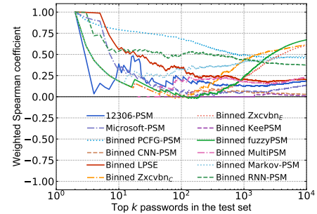
Figure 6: WSpearman of binned-PSMs under the knowledgeable online guessing strategy (tr: Rockyous, ts: LinkedIn). Binning degrades accurate PSMs while improving inaccurate ones. See Appendix F for more results.
