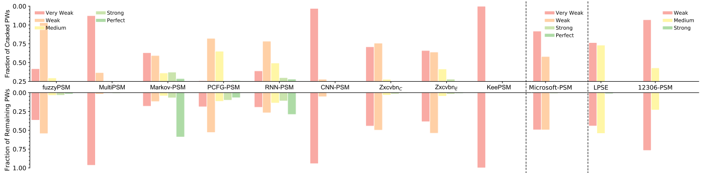
(c) Password score distributions (on Weibo) of leading PSMs under the probability-based guessing strategy.
