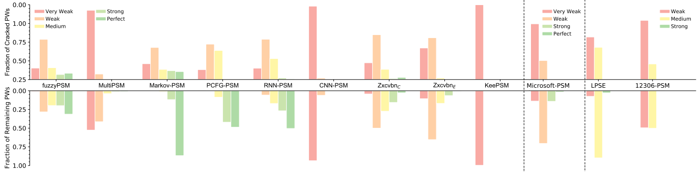
(c) Password score distributions (on LinkedIn) of leading PSMs under the probability-based guessing strategy.
