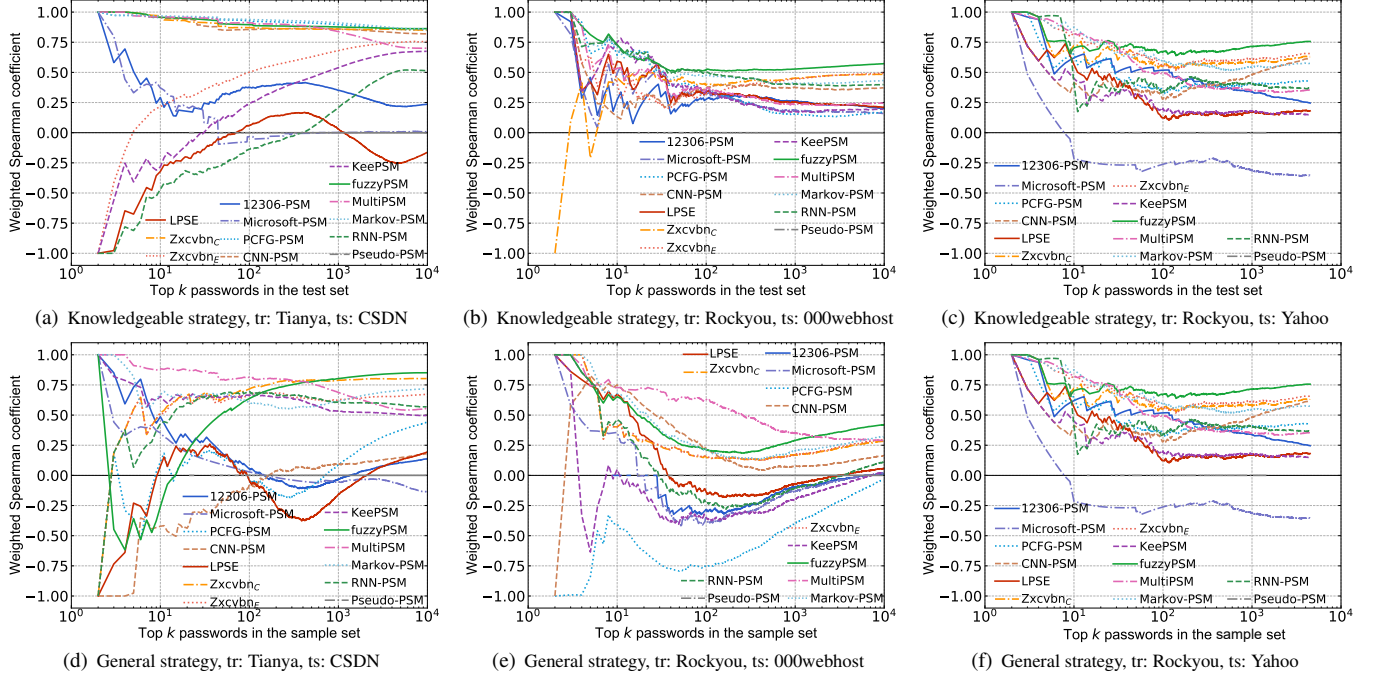
Figure 9: Weighted spearman correlation coefficient of state-of-the-art PSMs in online guessing scenarios (tr: Training set; ts: Test set).
