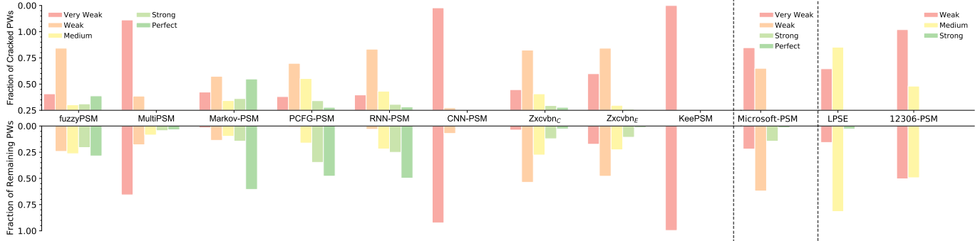
(b) Password score distributions (on LinkedIn) of leading PSMs under the dictionary-based guessing strategy.
