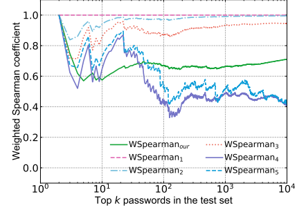
Figure 8: Results of our collected six different WSpearman calculation methods of Zxcvbn [14] on top-10 4 passwords in LinkedIn.
