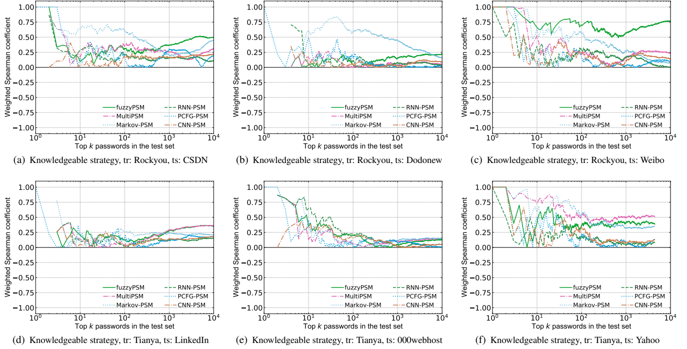
Figure 12: Influence of training set language on the accuracy of six attack algorithm-based PSMs under the knowledgeable online guessing strategy.
