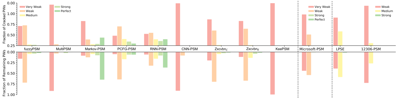
(b) Password score distributions (on Weibo) of leading PSMs under the dictionary-based guessing strategy.
