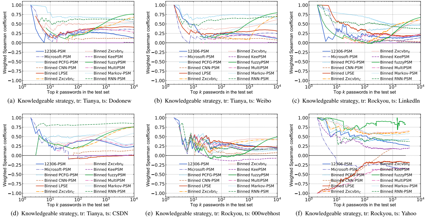
Figure 10: WSpearman of binned PSMs under the knowledgeable online guessing strategy (tr: Training set; ts: Test set).
