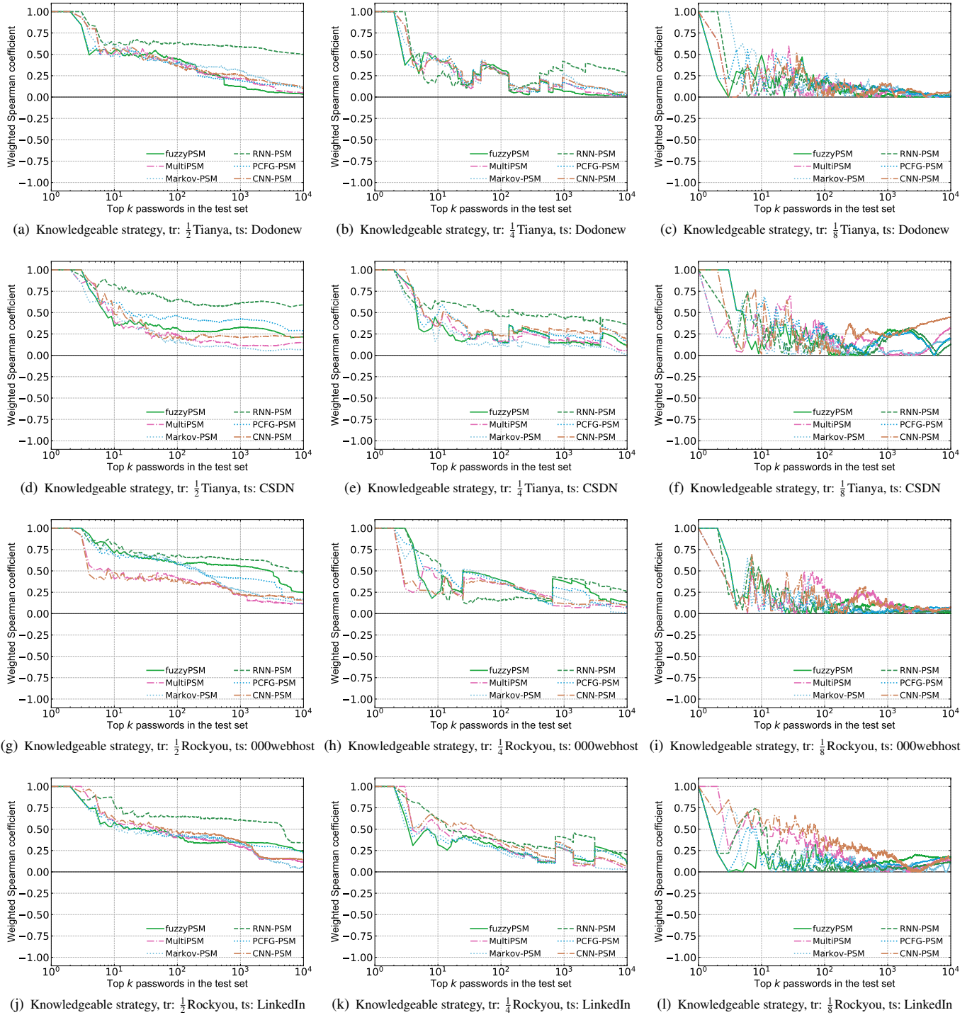
Figure 13: Influence of different training set sizes on the accuracy of six attack algorithm-based PSMs under the knowledgeable online guessing strategy.
