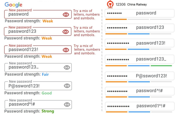
Figure 1: Inaccurate (see P@ssword123!) and inconsistent (see password123_) PSM feedback: Google ( https://myaccount.google.com/ ) and China Railway 12306 ( https://www.12306.cn/en/register.html ).
